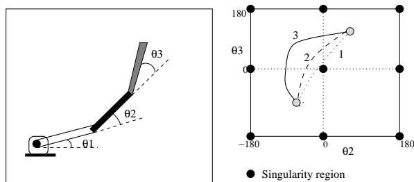
Figure 2: A 3-R manipulator
